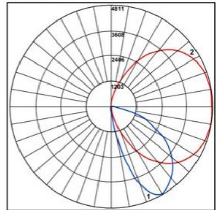
Maximum Candela = 4811 Located At Horizontal Angle = 10, Vertical Angle = 30 #1 - Vertical Plane Through Horizontal Angles (10-190) (Through Max. Cd.) #2 - Horizontal Cone Through Vertical Angle (30) (Through Max. Cd.)
